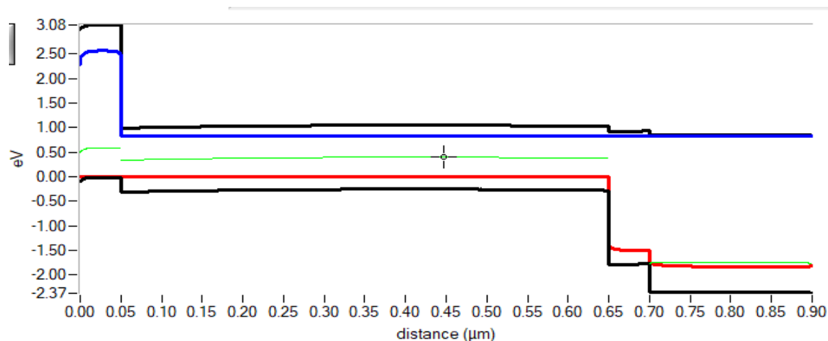
Fig.9 Energy Band Diagram of PSC with CuI HTL layer
