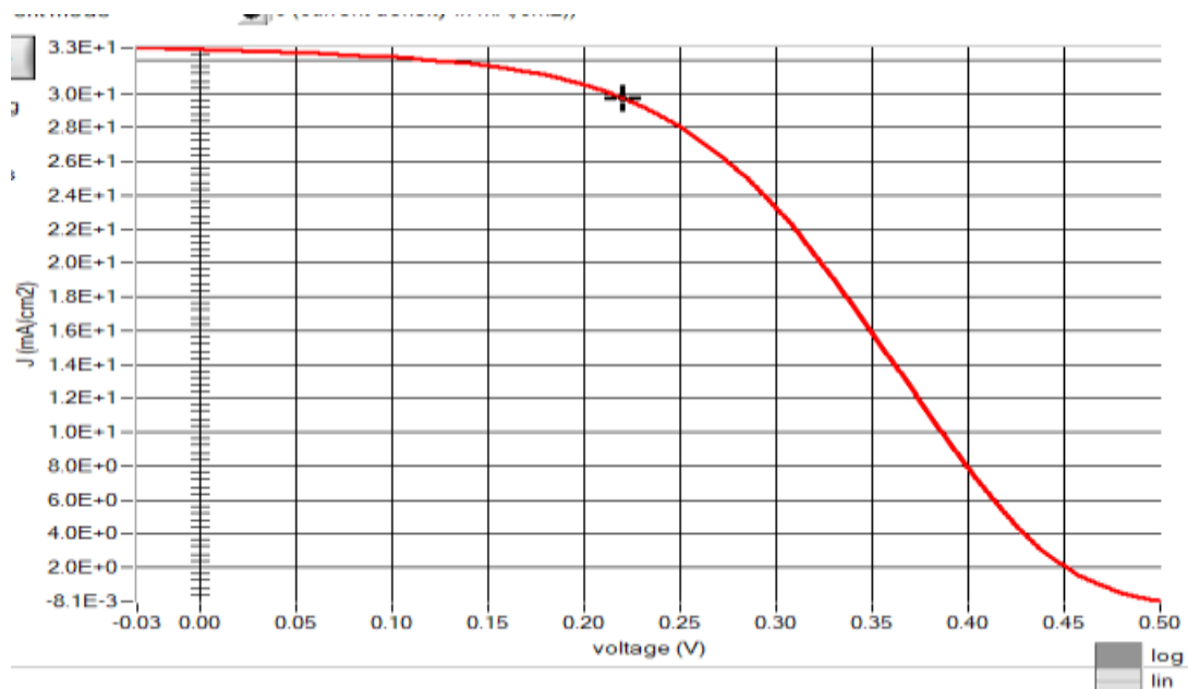
Fig.6 I-V Curve of PSC with PEDOT:PSS as HTL layer
