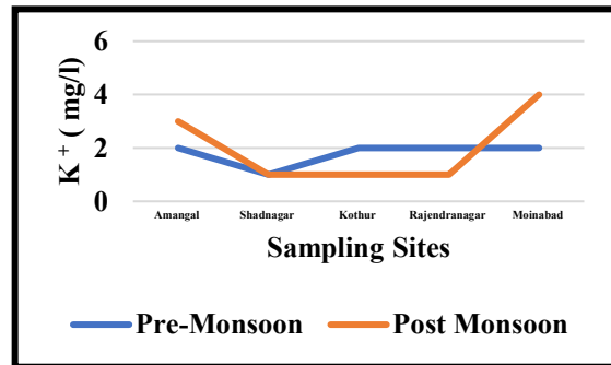
Amount of \text{K}^+ (mg/L) in Pre & Post Monsoon Season
